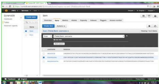
Figure7. Data in DynamoDB table after performing addition in balance
