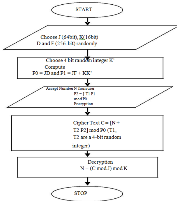
Figure3. Flowchart of Fully Homomorphic Encryption Scheme
