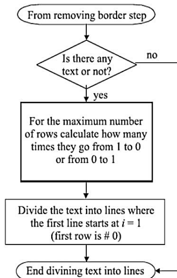
Figure 5. Converting Text into Lines Character
