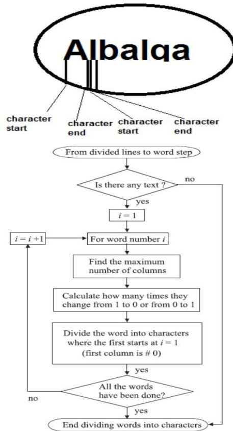
Figure 6. Character segmentation
