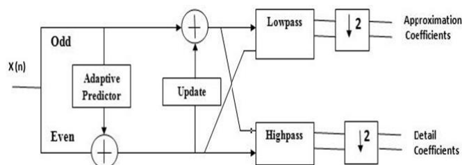
Figure 3. Forward multiwavelet transform using adaptive lifting scheme.
