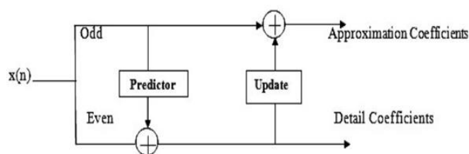
Figure 1. Convolution based lifting structure.
