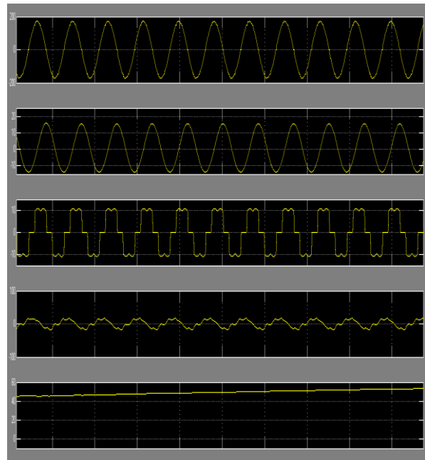
Figure 4. wave form representation of A Combination of Shunt Hybrid Power Filter and Thyristor-Controlled Reactor in steady state condition
