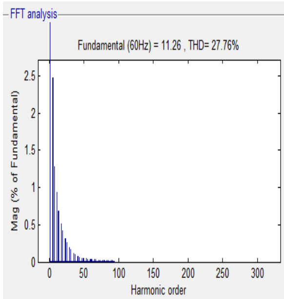
Figure 2. harmonic order for the conventional circuit configuration.
