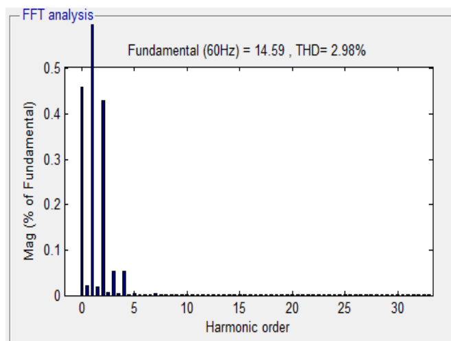
Figure 5. harmonic order A Combination of Shunt Hybrid Power Filter and Thyristor-Controlled Reactor in steady state condition
