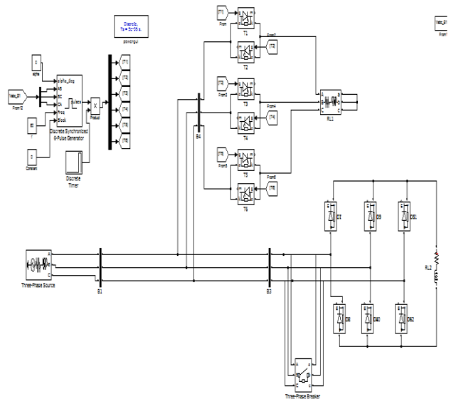
Figure 1. conventional circuit configuration
