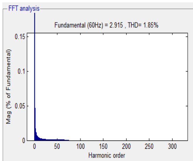
Figure 8. harmonic order A Combination of Shunt Hybrid Power Filter and Thyristor-Controlled Reactor in dynamic state condition
