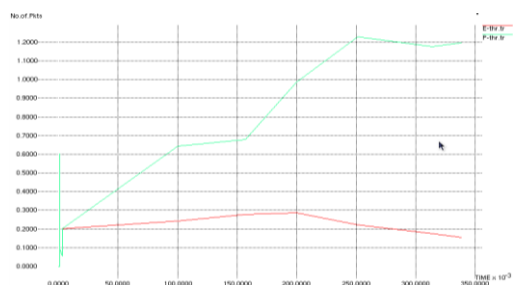
Figure 6 Throughputs vs. Time
