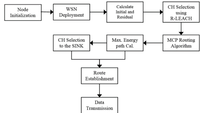
Fig. 1 MCP Routing method
