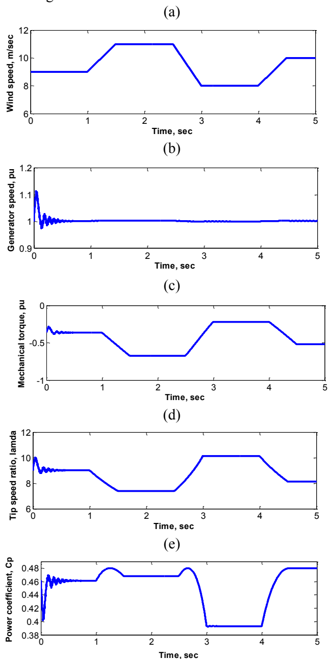
Figure 6. Constant speed System response for ramp changes in wind speed
