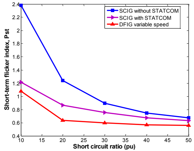
Figure 9. The effect of SCR on the short-term flicker index P_{st} .
