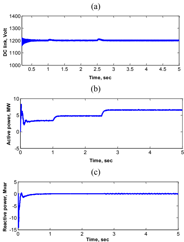
Figure 5. Grid side converter response for step changes in wind speed
