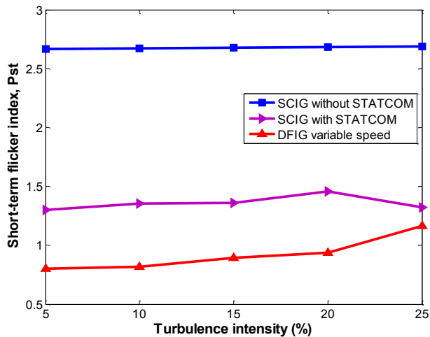
Figure 12. Variation of P_{st} with wind speed turbulence.
