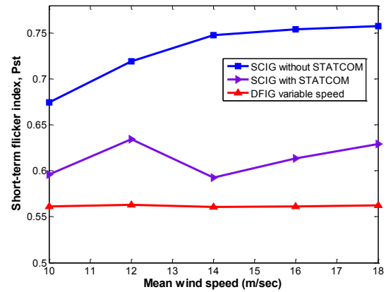
Figure 11. Variation of P_{st} with the mean wind speed
