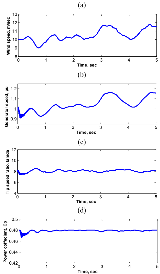
Figure 8. Variable speed System response for random changes in wind speed
