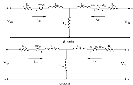
Figure 3. The d-q equivalent circuit of DFIG [1].
