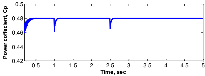
Figure 4. Rotor side converter response for step changes in wind speed
