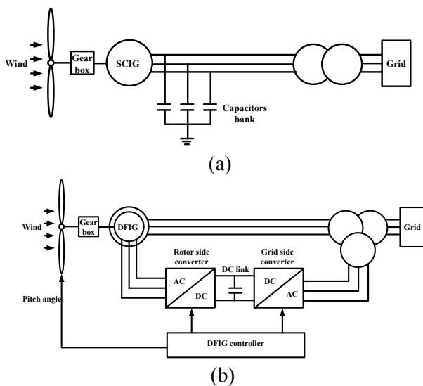
Figure 1. (a) Constant speed SCIG directly grid connected wind turbines
