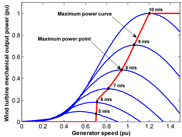
Figure 2. Wind turbine mechanical power output rotor speed [12].
