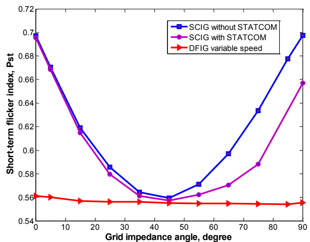
Figure 10. Variation of P_{st} with the grid impedance angle
