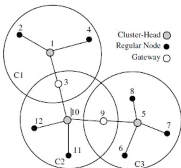
Figure 2. Illustration of a typical cluster-based network.
