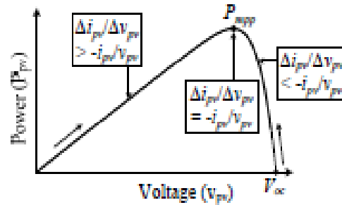
Figure 3. illustration of INC_MPPT with SPV array Ppv-Vpv characteristics.
