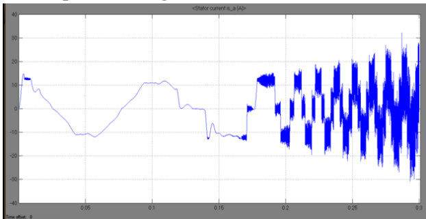
Motor stator current Ia
