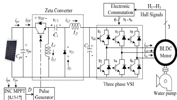
Figure 2. Proposed solar PV-zeta converter fed BLDC motor drive for water pump.
