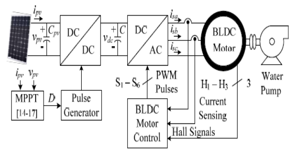
Figure 1. Conventional SPV fed BLDC motor driven water pumping system.
