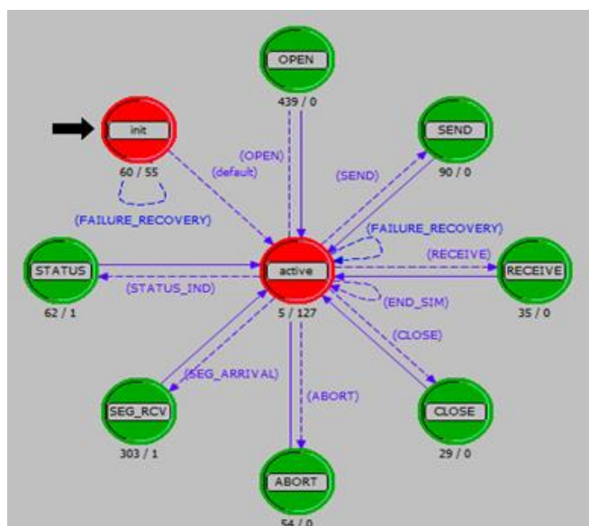
Figure 1. Process Model of TCP Manager
