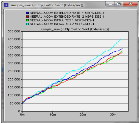
Figure 4. Sample Sum for FTP Traffic Sent (bytes/sec) in 1&2 Mbps for IRWLAN and Extended Rate 802.11g
