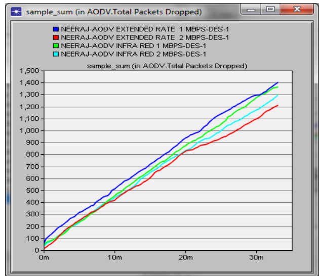
Figure 6. Sample Sum for AODV Packets Dropped Total (bits/sec) in 1&2 Mbps for IRWLAN and Extended Rate 802.11g
