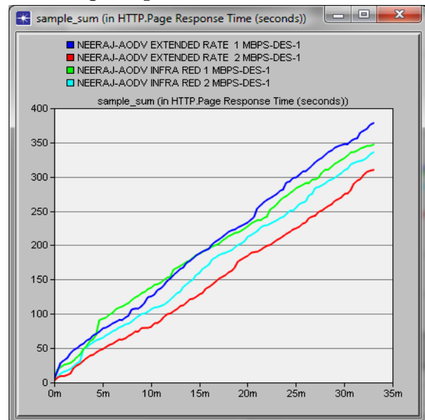
Figure 3. Sample Sum for HTTP Page Response Time (sec) in 1&2 Mbps for IRWLAN and Extended Rate 802.11g
