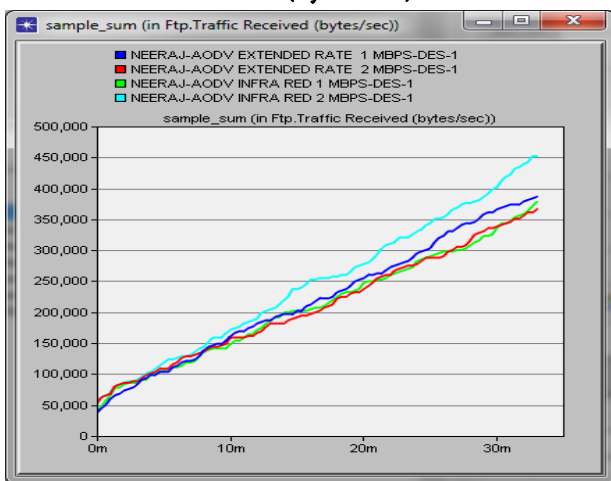
Figure 5. Sample Sum for FTP Traffic Received (bytes/sec) in packets in 1&2 Mbps for IRWLAN and Extended Rate 802.11g
