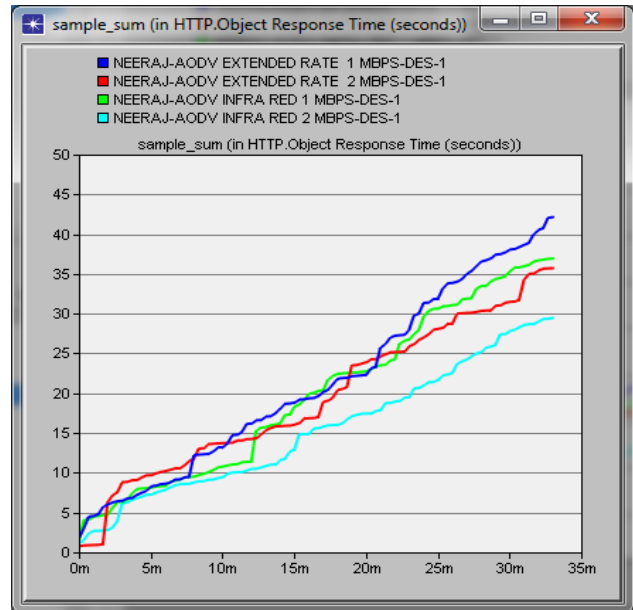
Figure 2. Sample Sum for HTTP Object Response Time (sec) in 1&2 Mbps for IRWLAN and Extended Rate 802.11g
