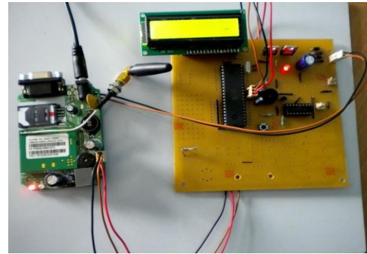
Figure 3. Prototype board showing GSM module and LCD display.
