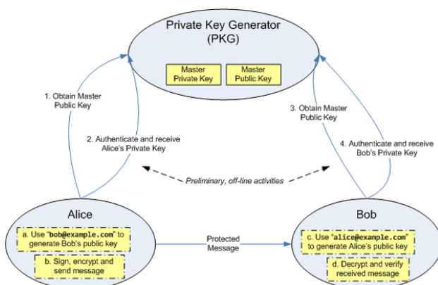
Figure 1. Working of IBE System
