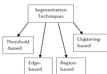
Fig.2.egmentation techniques.
