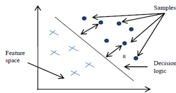
Figure 1 : SVM Classifier
