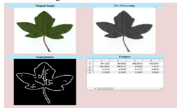
Figure 4: ANN Results
