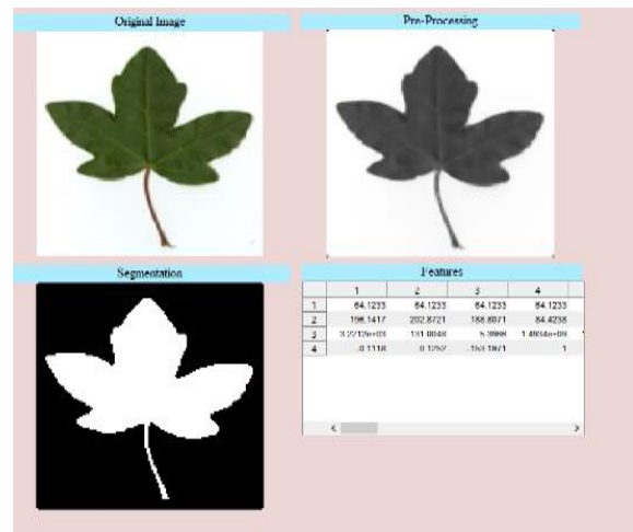
Figure 4: ANN Results
