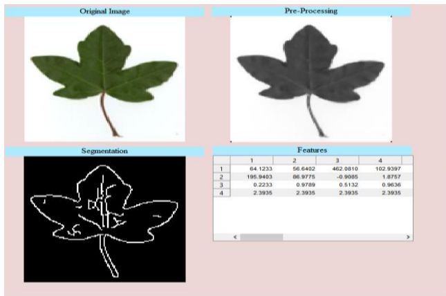
Figure 6 : Proposed System with Random Forest Classifier
