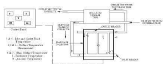
Figure 2. Experimental Setup
