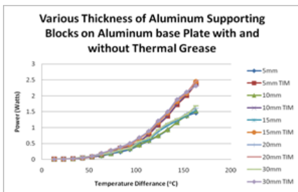
Graph 1.2: Power (Watts) vs Temperature difference (°C)
