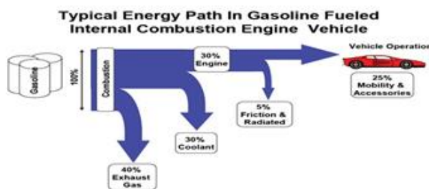
Figure 1.1: Typical energy path in gasoline fuelled internal combustion engine vehicles [8].
