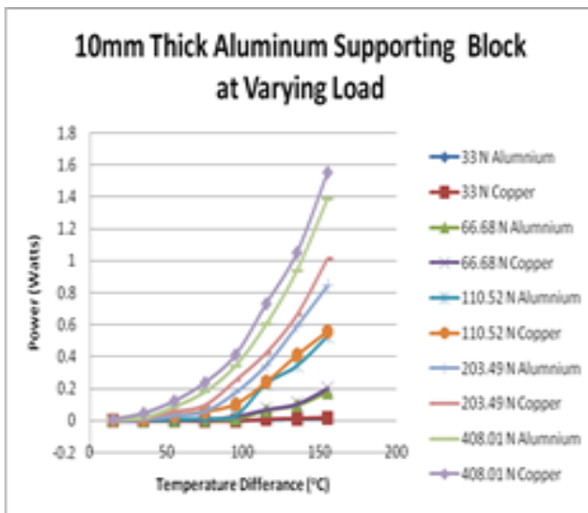
Graph 1.1: Power (Watts) vs Temperature difference (oC)
