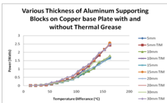
Graph 1.3: Power (Watts) vs Temperature difference (°C)
