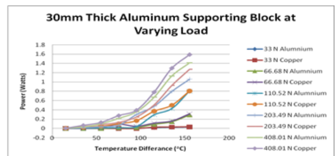
Graph 1.1: Power (Watts) vs Temperature difference (oC)
