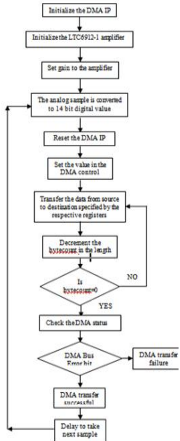
Figure 6: Flow Diagram of DMA transfer implementation [6]
