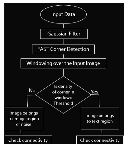
Fig.4: Flow chart for the algorithm[8]
