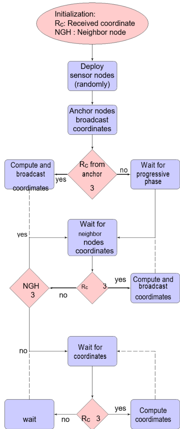
Fig. 2. Flowchart of Proposed Mechanism
