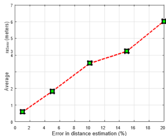
Fig. 7. The performance of proposed approach with varying error in distance estimation observed that the localization error increases with increase in measurement error in distance estimation as shown
