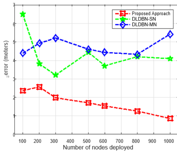
(a) Area 50x50 m 2
