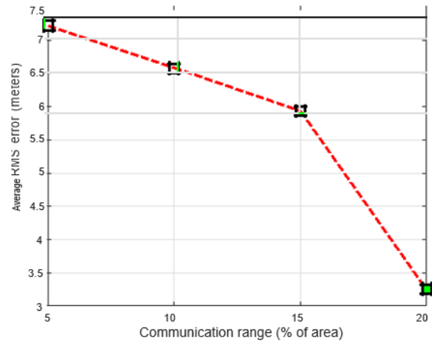
Fig. 5. The performance of proposed approach with varying communication range ten anchor nodes are deployed in 100m 100m area. The error in the distance is considered as 10% of the respective distance.
