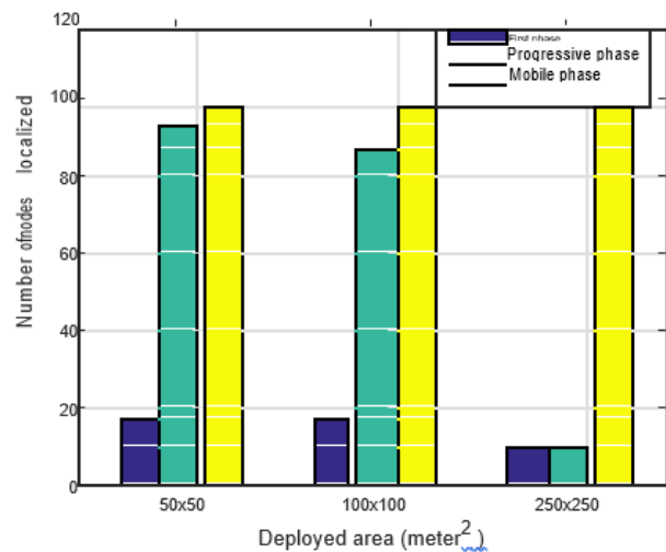
(b) Total node localized
