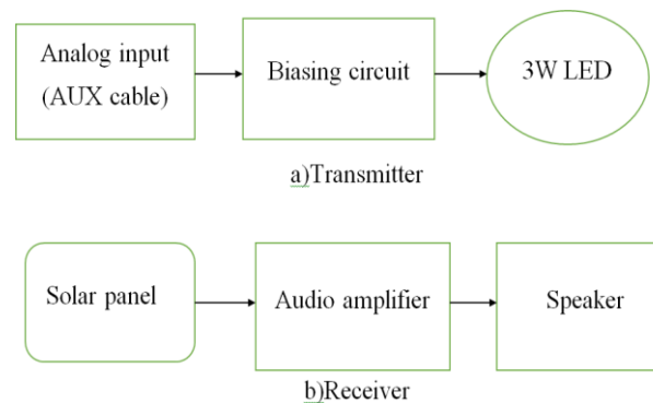
Figure 6. Block Diagram of proposed audio transfer system
