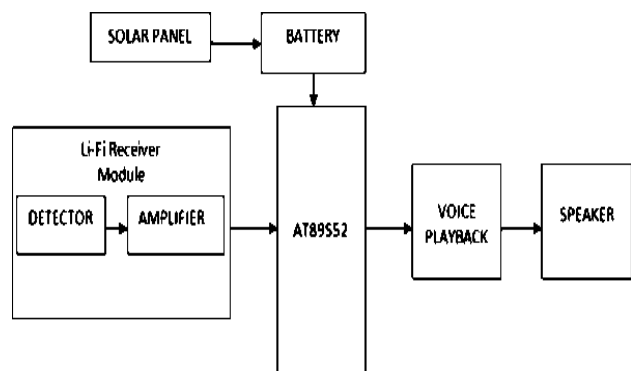
Figure 2. Receiver block diagram using Atmel
