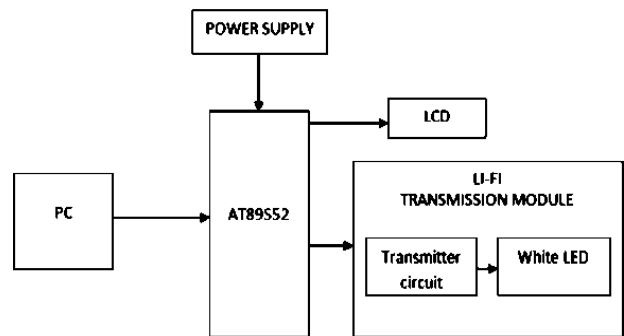
Figure1. Transmitter block diagram using Atmel
