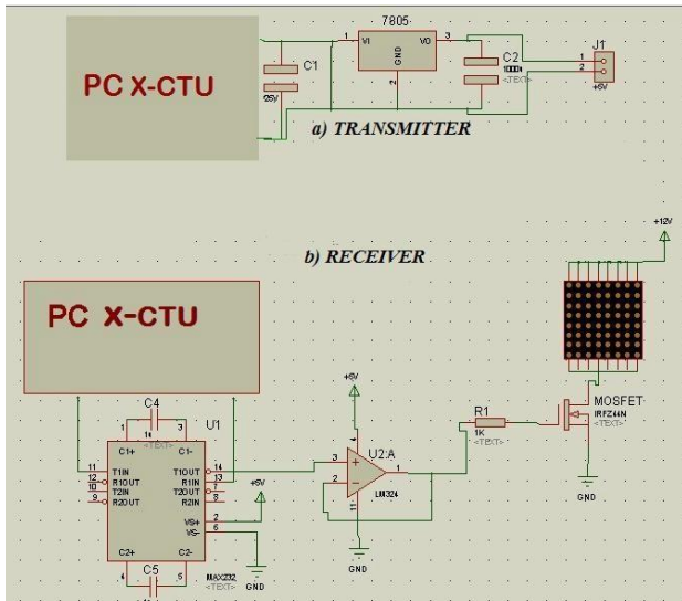
Figure 5. Circuit diagram of proposed data transfer system
