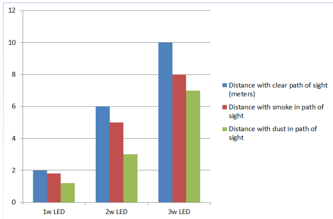
Figure 7. Comparison of different LEDs and distance travelled by light ray under different conditions
