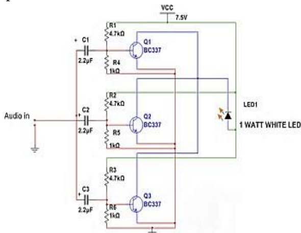
Figure 3. Audio Transmitter Circuit
