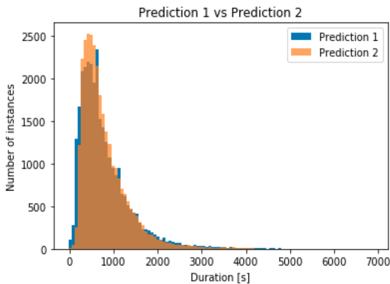
Fig 5: Comparison between the Predicted and Testing Data
