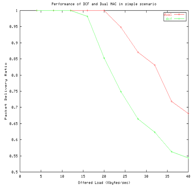
Fig 4: Packet Delivery Ratio for Dual MAC Vs DCF MAC in simple scenario
