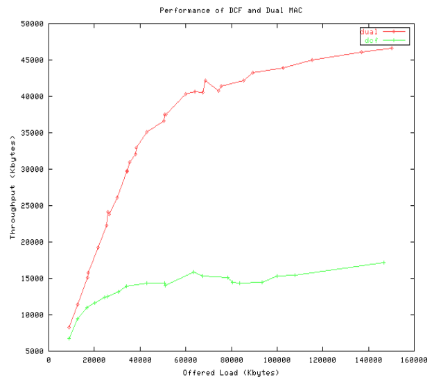
Fig 5: Dual MAC Vs DCF MAC – overall
