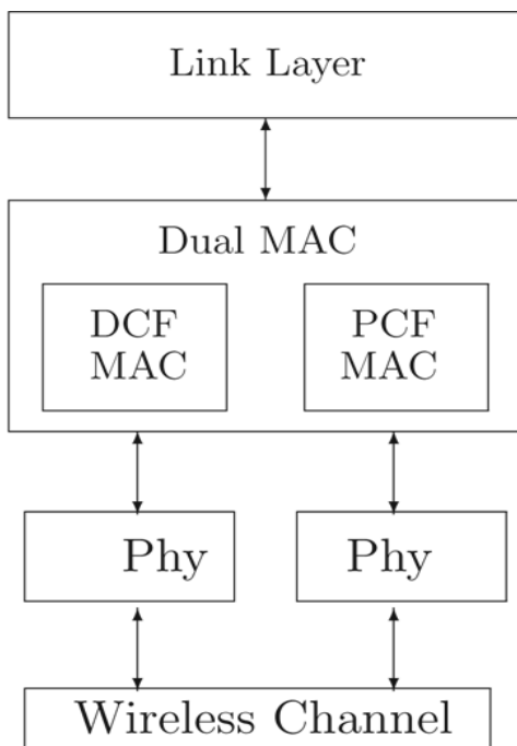
Fig. 1: Architecture of Dual MAC
