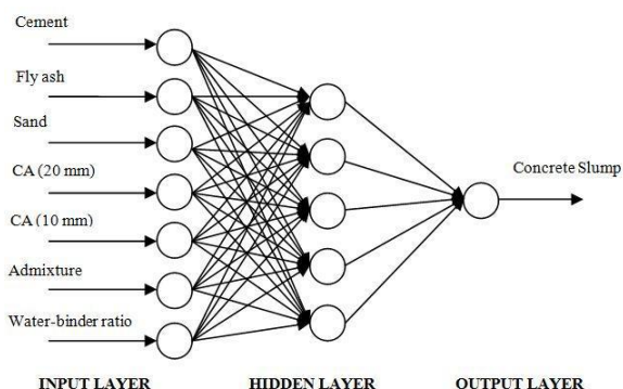
Figure 1 Three layer feed forward neural network
