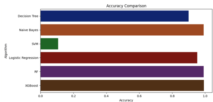
Fig 2 : Accuracy Comparison
