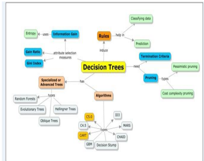
Figure 1. Working Process for DT algorithm
