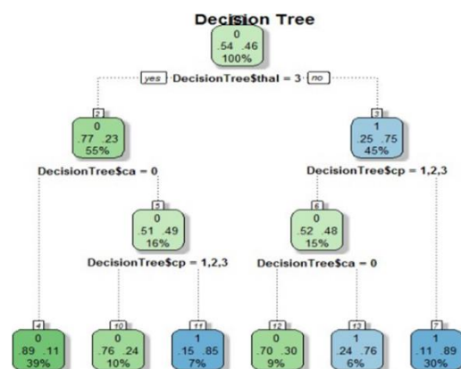
Figure 3. DT for the given Data Set
