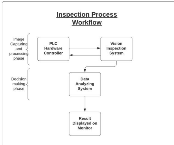
Fig 5: Workflow of Inspection Process
