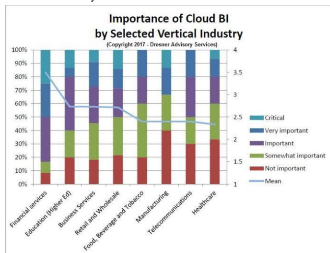
Figure 6: Importance of cloud BI in selected vertical industry in 2017 [12].
