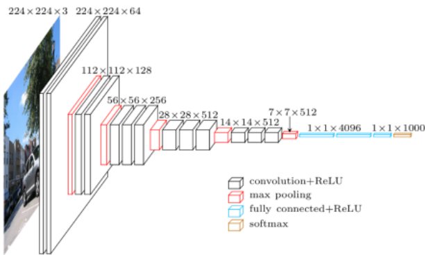
Fig.1. Architecture of VGG-16
