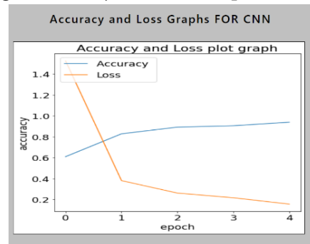
Fig.6 Accuracy and Loss Graphs for CNN
