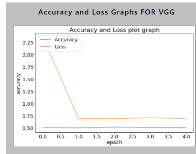
Fig.5 Accuracy and Loss Graphs for VGG
