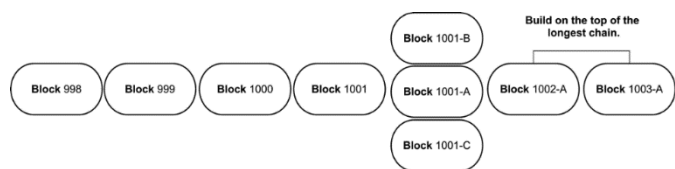
Figure 7. Longest Chain Rule
